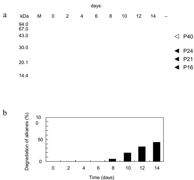
Figure 2 a, Induction of P24, P21 and P16 productions in G. thermoleovorans B23. Cells were cultivated in LBM supplemented with 0.1% alkane mixtures (V/V) for 14 days at 70°C. Total cell fractions were loaded on an SDS-12% polyacrylamide gel. Protein bands were stained with Coomassie Brilliant Blue R-250. Lanes are molecular size marker, M; cultures after 0 day, 0; 6 days, 6; 8 days, 8; 10 days, 10; 12 days, 12; 14 days, 14; and 14 days cultivation in the absence of alkanes, -. b, Relative degradation of alkanes by strain B23. Fractions degraded were estimated by the reduction of peak areas in GC/FID.
