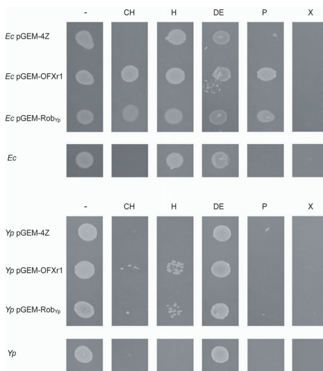
Figure 4 Effect of robA Yp overexpression on organic solvent tolerance. Cultures of Y. pestis ( Yp ) and E. coli ( Ec ) strains carrying the plasmids indicated were spotted on solid medium. The surface of the medium was overlaid with the organic solvent and growth was recorded after incubation. H, n -hexane; CH, cyclohexane; P, n -pentane; X, p -xylene; DE, diphenyl ether; -, no solvent control.
