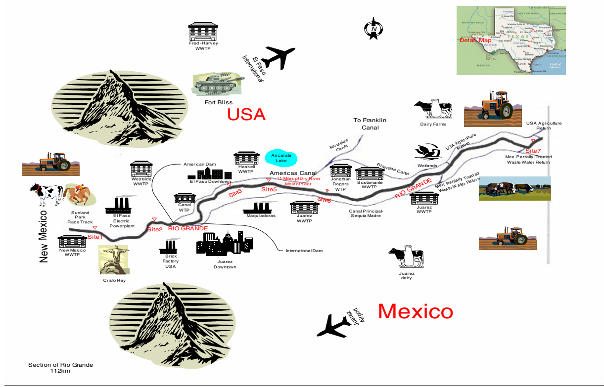
Figure 1 Sampling Locations in the Rio Grande basin.
