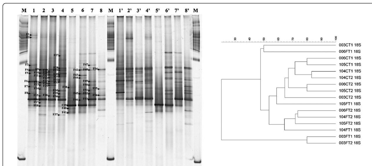
Figure 3 Denaturing gradient gel electrophoresis (DGGE) fingerprints of fungal 18S rRNA gene fragments amplified from stem and leaf DNA templates obtained from four genotypes of Lippia sidoides using two sets of primers - EF4/ITS4 [27,28] and ITS1f/ITS2 [24,25]. Lanes 1, 2, 3, 4, 1', 2', 3', 4' – stem samples and 5, 6, 7, 8, 5', 6', 7', 8' – leaf samples from genotypes LSID003, LSID006, LSID104 and LSID105, respectively. Lanes marked with M correspond to a 1 kb ladder (Promega). The letter F followed by numbers indicates bands that were extracted from the gels for sequence analysis. The right side shows the corresponding dendrogram obtained after cluster analysis with mathematical averages (UPGMA) and Dice similarity coefficients comparing the fungal 18S rRNA gene fragments amplified from stem and leaf DNA templates obtained from four genotypes of L. sidoides . The genotypes are represented by the three first numbers (LSID - 003, 006, 104 and 105), followed by C or F for stem and leaf samples, respectively, and T1 and T2 corresponding to the replicates.
