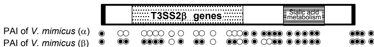
Figure 2 Comparison of the structure of PAI in V. parahaemolyticus , V. cholerae and V. mimicus . Schematic representation of the structure of the PAI in V. parahaemolyticus RIMD2210633 (containing T3SS2 \alpha ) and TH3996 (containing T3SS2 \beta ) strains and in V. cholerae AM-19226 (containing T3SS2 \alpha ) and 1587 (containing T3SS2 \beta ) strains. Names of the various V. parahaemolyticus and V. cholerae strains are shown along the left side. Black boxes represent core chromosomal genes flanking the PAI region in V. parahaemolyticus or V. cholerae strains. Horizontally striped boxes represent sialic acid metabolism regions, and the checkered box represents the urease gene cluster, while diagonally striped and dotted boxes represent T3SS2 regions, and white boxes other ORFs in PAI regions. White circles represent the ORFs which were tested for the presence or absence of ORFs in V. mimicus strains, and black circles indicate the presence of such ORFs.
